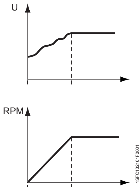
Figure 7.15: The function of Torque Control during start
